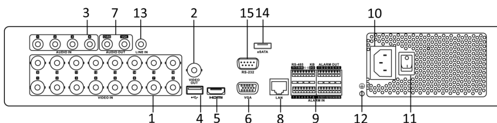
Figure 1-12 Rear Panel of DS-7300HQHI-K
