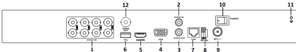
Figure 1-11 Rear Panel of DS-7200HQHI-K/P
