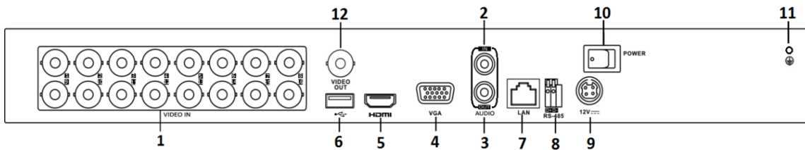
Figure 1-10 Rear Panel of DS-7200HQHI-K
