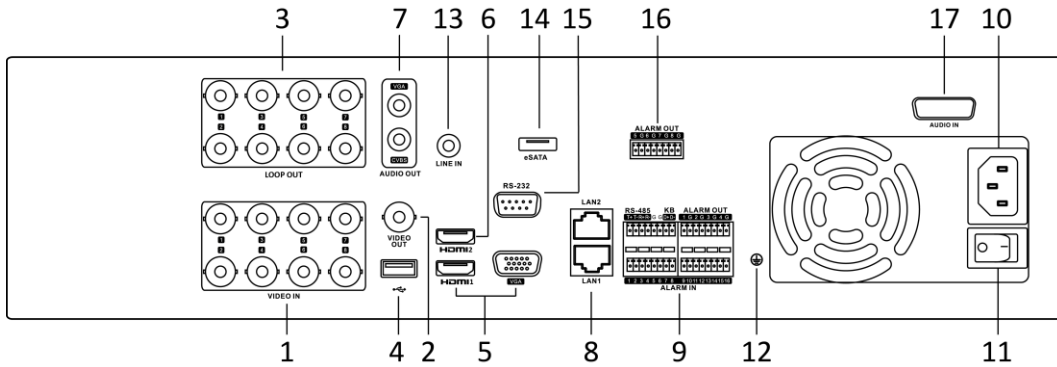
Figure 1-14 Rear Panel of DS-9000HUHI-K8
