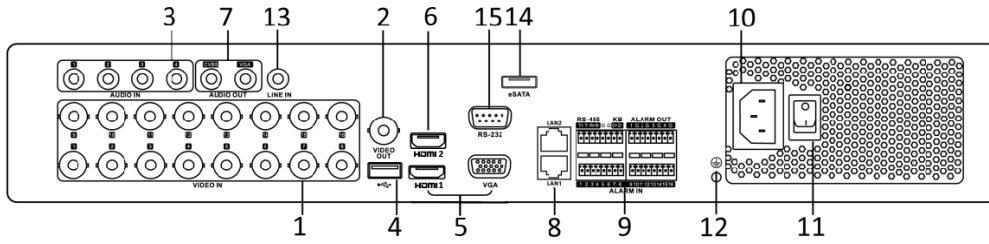
Figure 1-13 Rear Panel of DS-7300HUHI-K4
